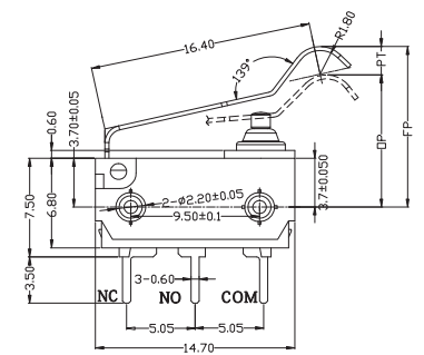
22# Lever
