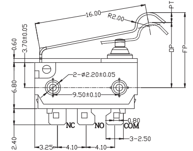
41# Lever
