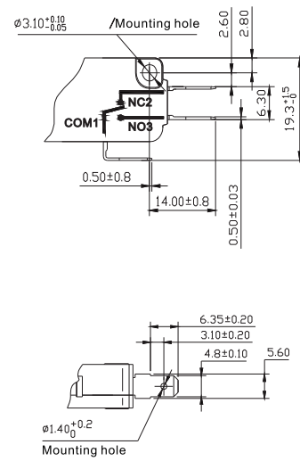
E1 Flat Type Housing with 187# Quick Connect Terminals, T=0.5(E1)
