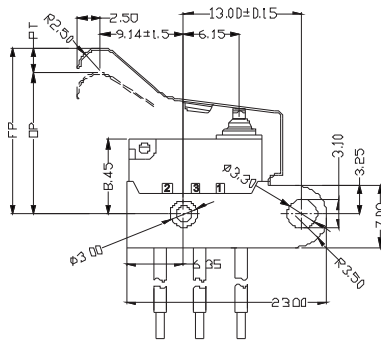
10# Lever
