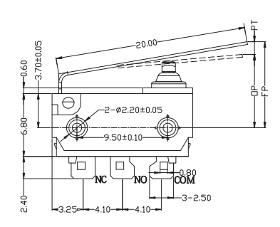
28# Lever
