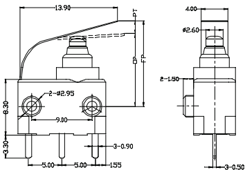
03 Straight leaf lever
