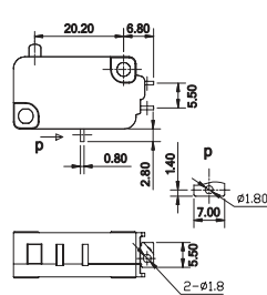
P Straight PCB Terminal
