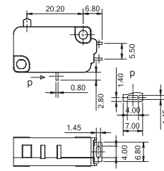
K Rectangle Hole Solder Terminal
