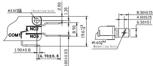
E2 Fully Flat Type Housing with 187# Quick Connect Terminals, T=0.5(E2)
